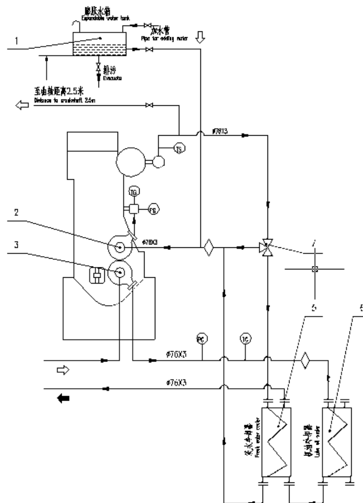
Cooling System Schematic Diagram
