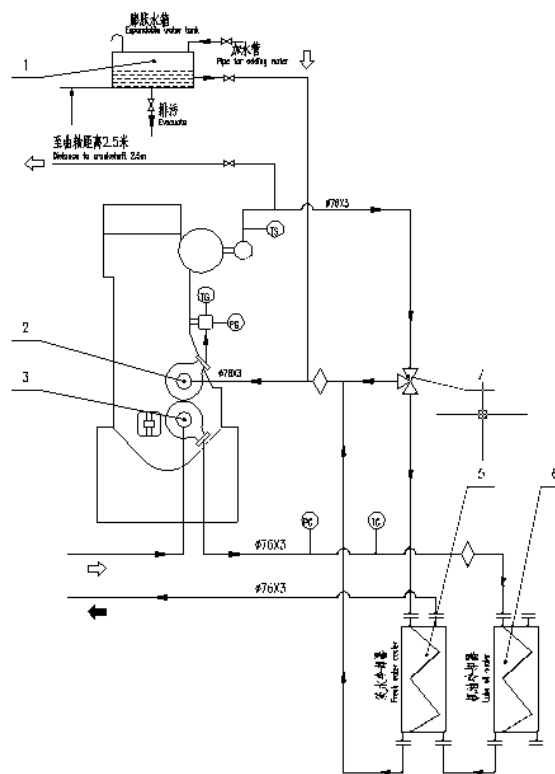
Cooling System Schematic Diagram
